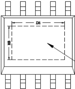
HEAT SLUG
